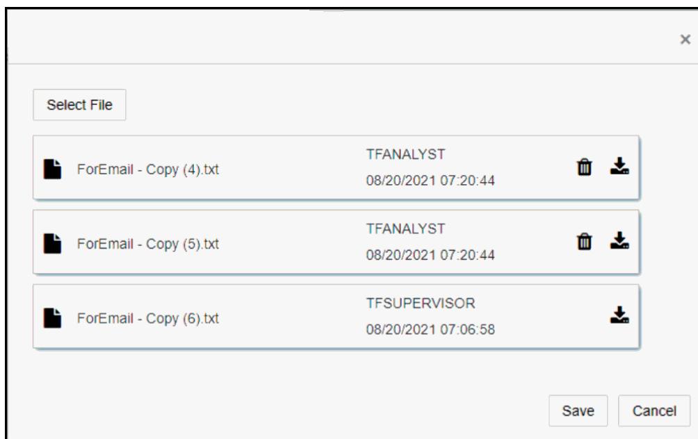
Figure 12: Add Attachments
